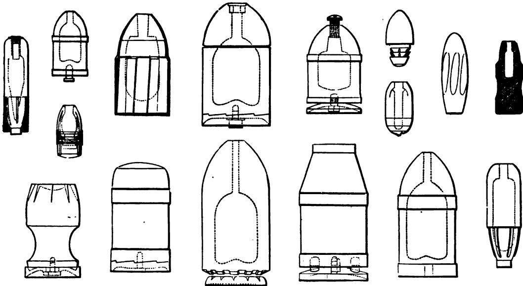
VARIOUS FORMS OF PROJECTILES USED IN THE AMERICAN WAR.
